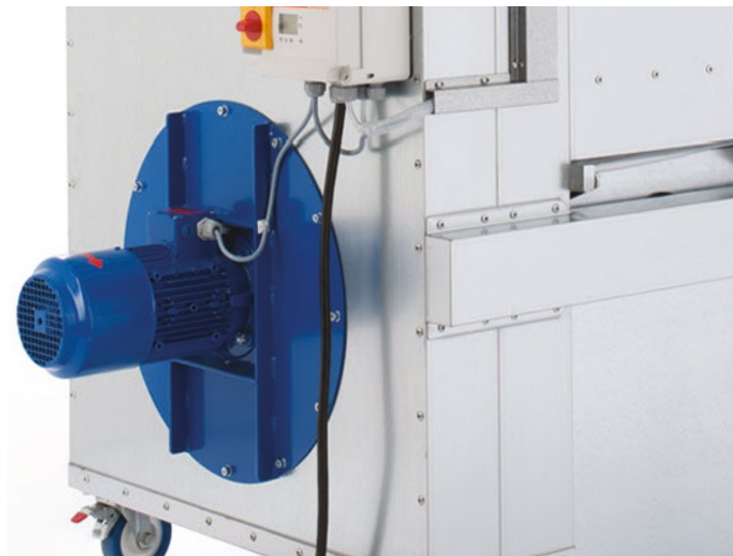
Illustration above: Vacumobil VT 160 with 2.2 kW energy-saving motor (IE4)
